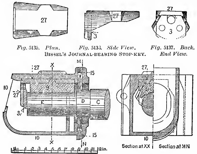
Fig. 5133. Section. Fig. 5134. BISSEL'S STOP-KEY JOURNAL BEARINGS FOR COLLARLESS JOURNALS.
